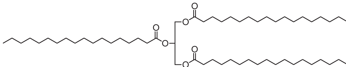
Structure A
