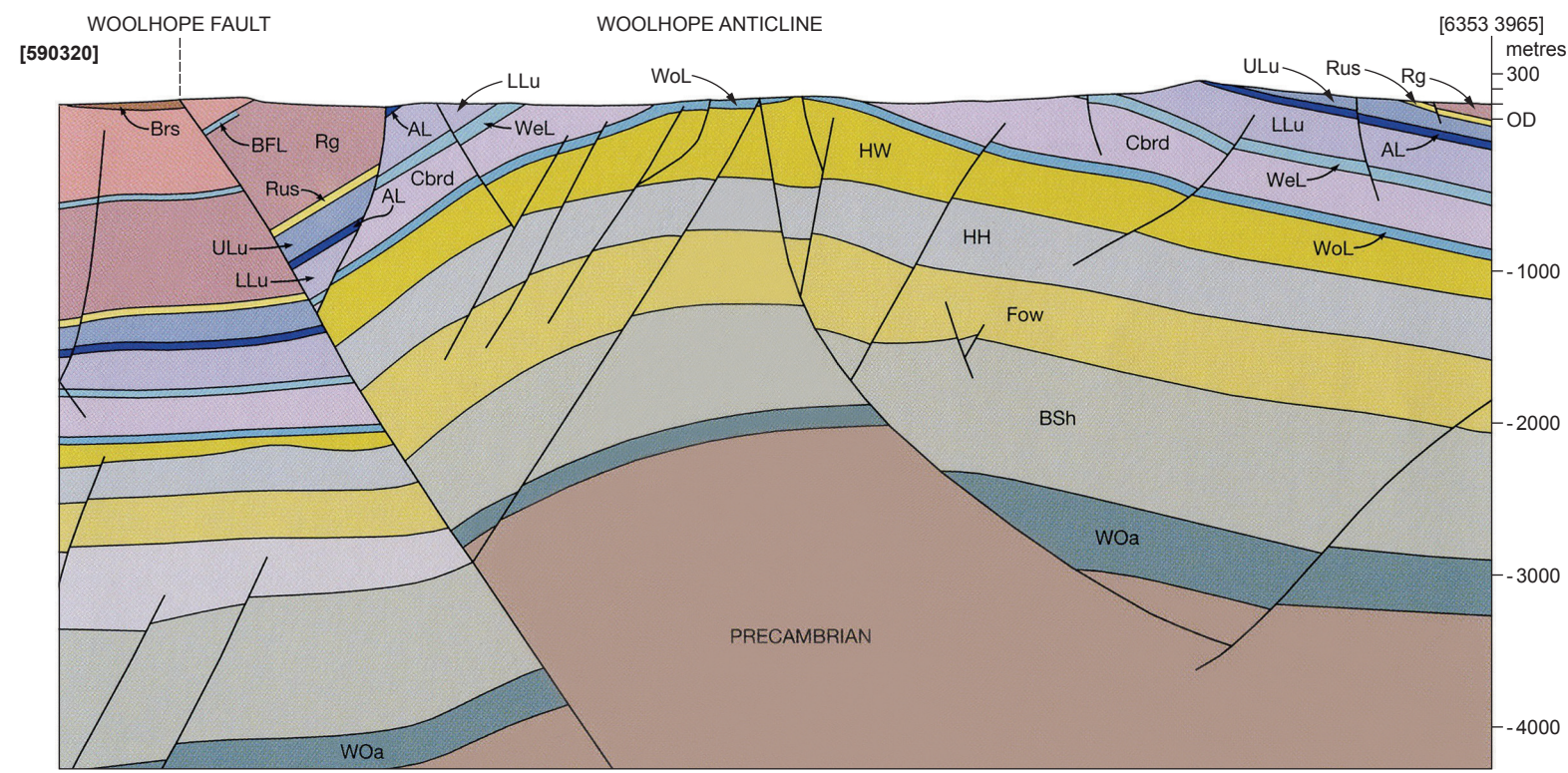
CROSS-SECTION SHOWING THE GENERAL RELATIONS OF THE ROCKS ALONG THE LINE DRAWN ON THE MAP Horizontal and Vertical scales 1:50 000
